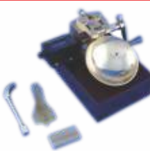
LIQUID LIMIT DEVICE (HAND)
